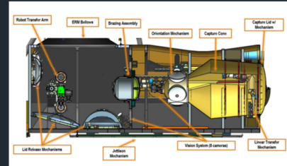
Capture and Containment Module (CCM)
