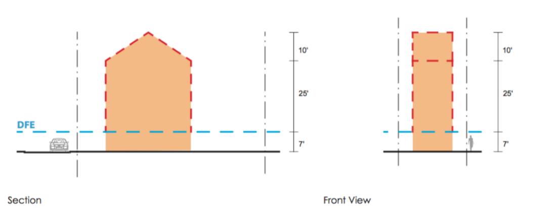
R4 requirements on typical Gerritsen Beach lots of 24' x 66'
