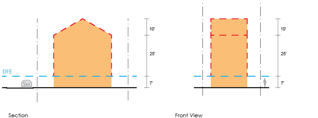
R4 requirements on typical Gerritsen Beach lots of 40' x 45'
