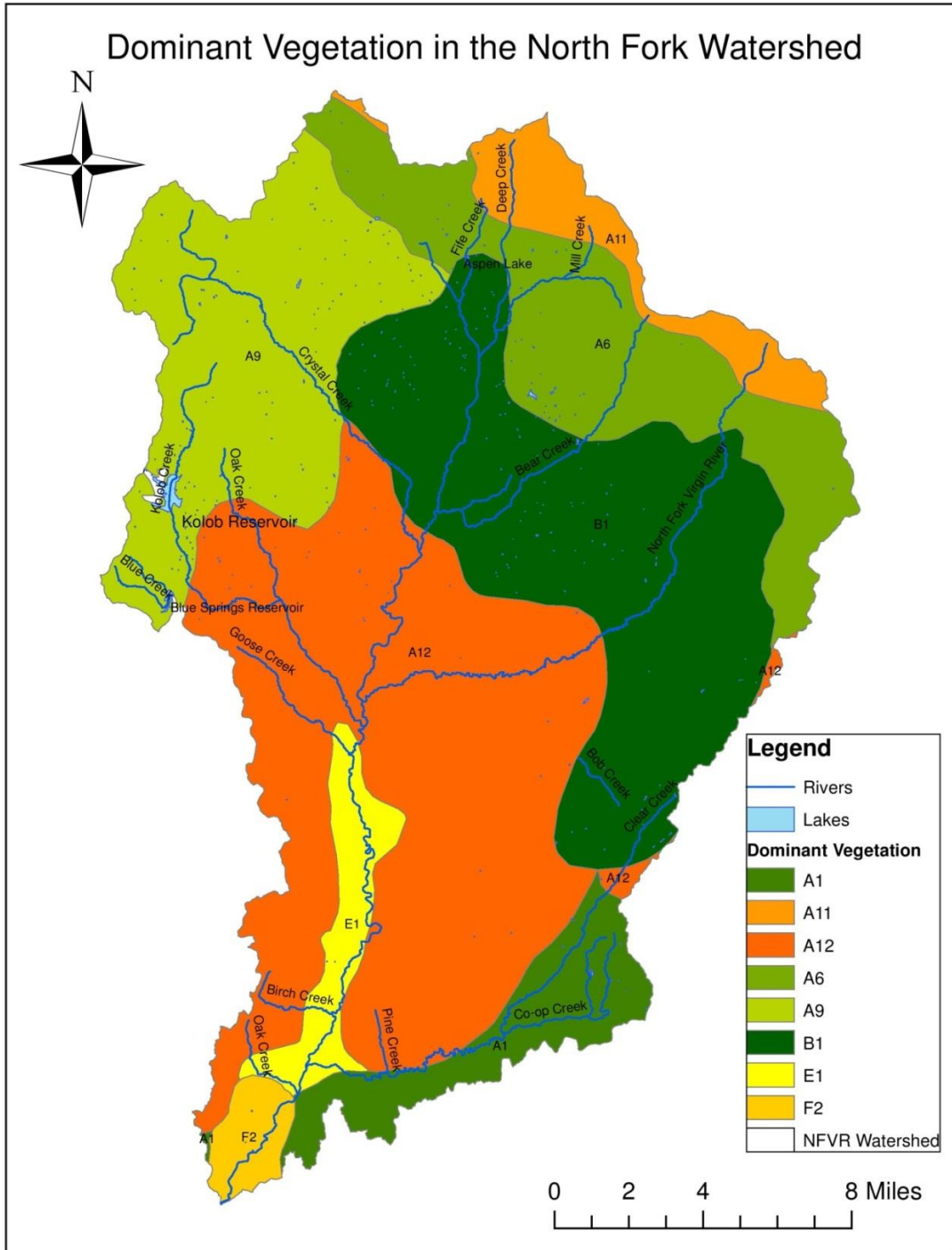
Map 5: Dominant Vegetation in the North Fork Virgin River Watershed (refer to Table 7 for a description of dominant vegetation symbols)
