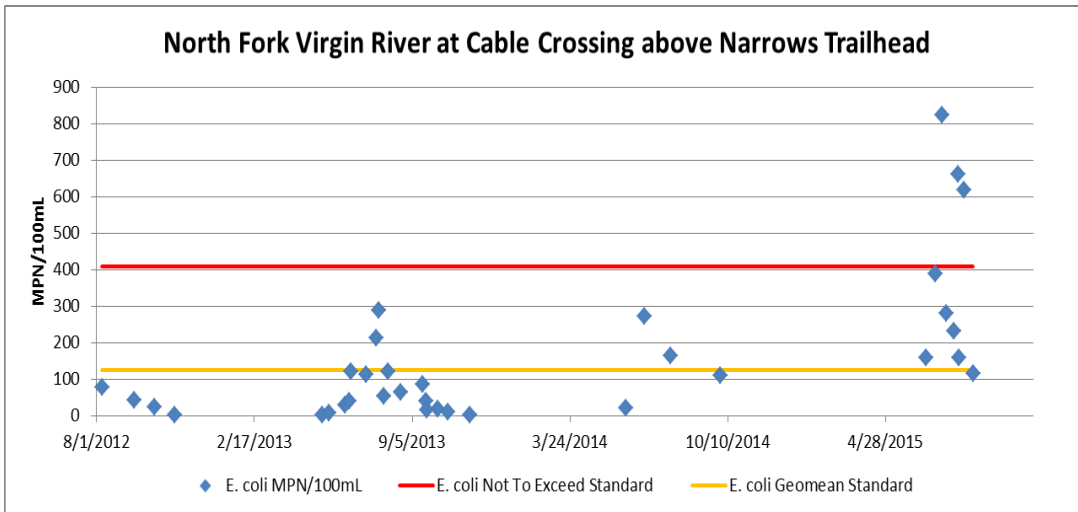
Figure 12: E. coli concentrations measured at North Fork Virgin River at cable crossing above Zion Narrows trailhead from 2012-2015.
