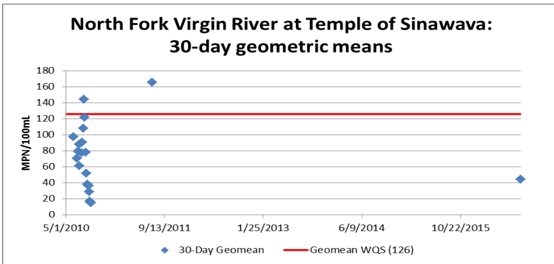
Figure 23: 30-day geometric means of E. coli concentrations for North Fork Virgin River at End of Road site
