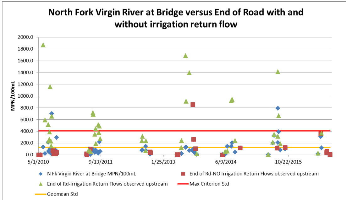
Figure 18: E. coli concentrations at Bridge site versus End of Road site with and without return flow.
