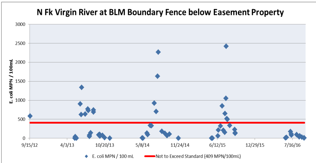
Figure 40: E. coli concentrations below Conservation Easement property
