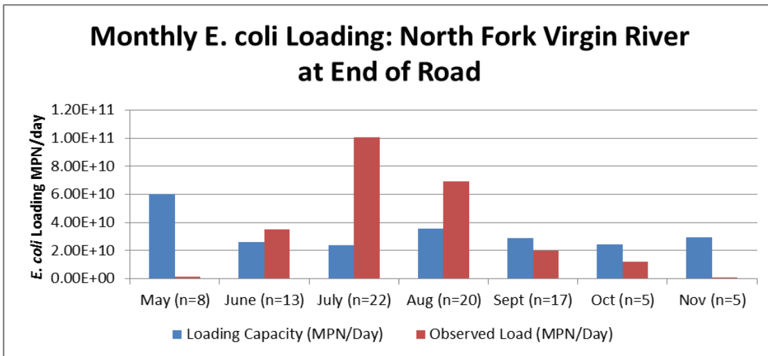
Figure 29: Monthly loading capacity versus observed loading at End of Road monitoring site
