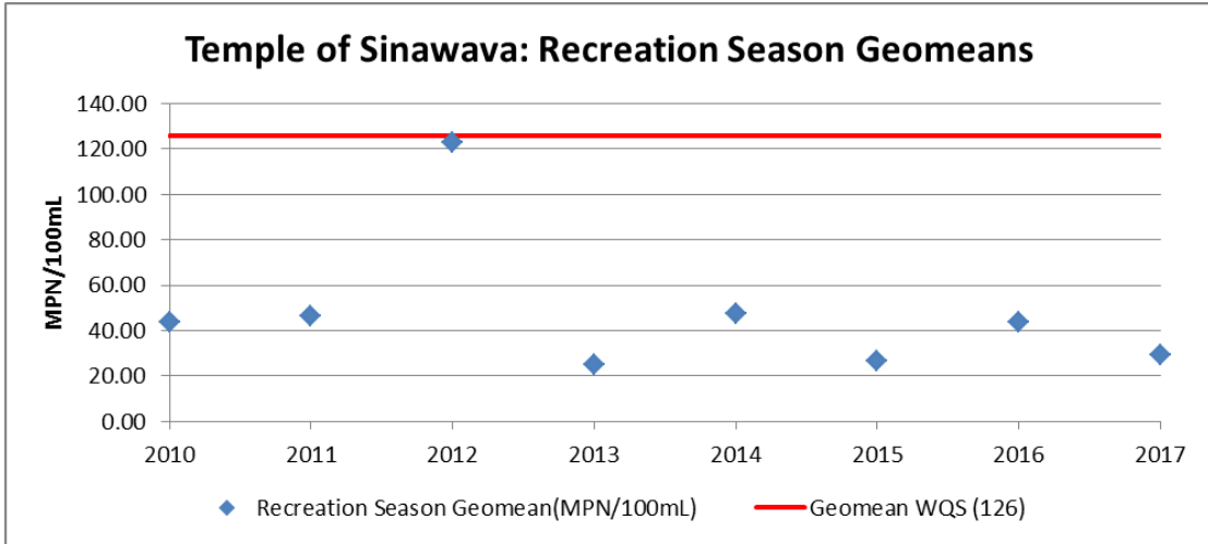
Figure 24: Geometric means of E. coli concentrations during recreation season (May-October) from 2010-2017 at North Fork Virgin River at Temple of Sinawava site
