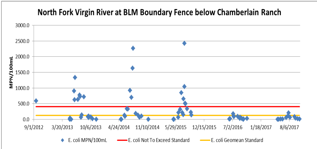
Figure 15: E. coli concentrations measured at North Fork Virgin River at BLM Boundary Fence below Chamberlain Ranch from 2012-2017.
