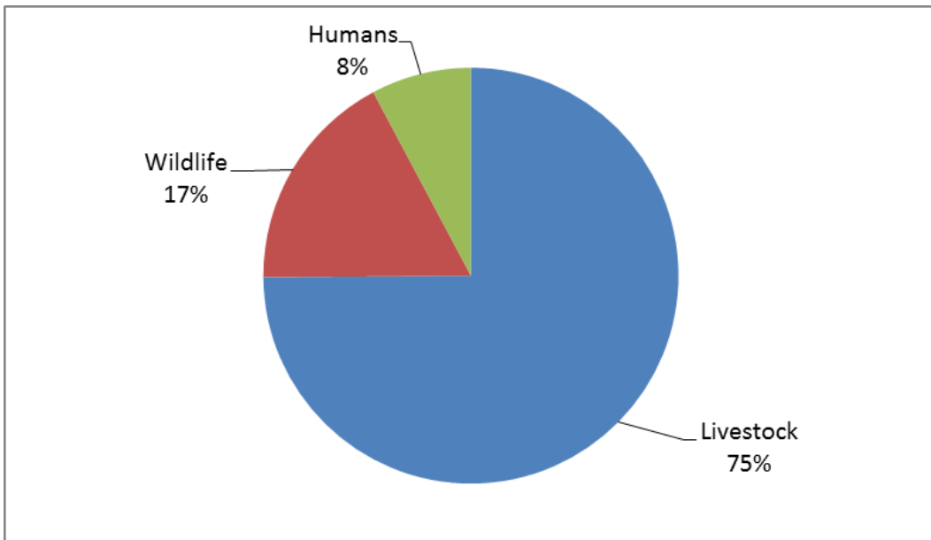
Figure 34: Estimated bacteria contribution by source during the recreation season.
