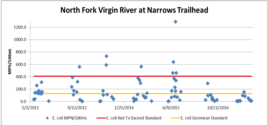
Figure 14: E. coli concentrations measured at North Fork Virgin River at Zion Narrows Trailhead from 2011-2017.
