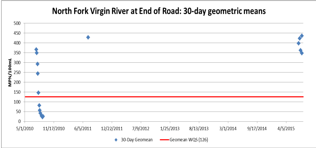
Figure 20: 30-day geometric means of E. coli concentrations for North Fork Virgin River at End of Road site
