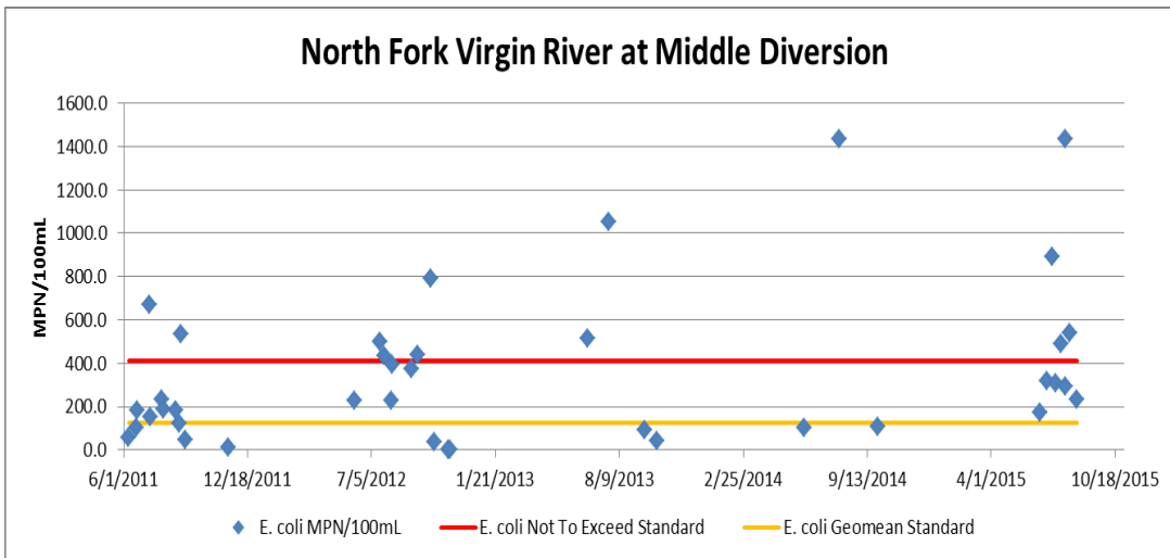
Figure 16: E. coli concentrations measured at North Fork Virgin River at Middle Diversion from 2011-2015.
