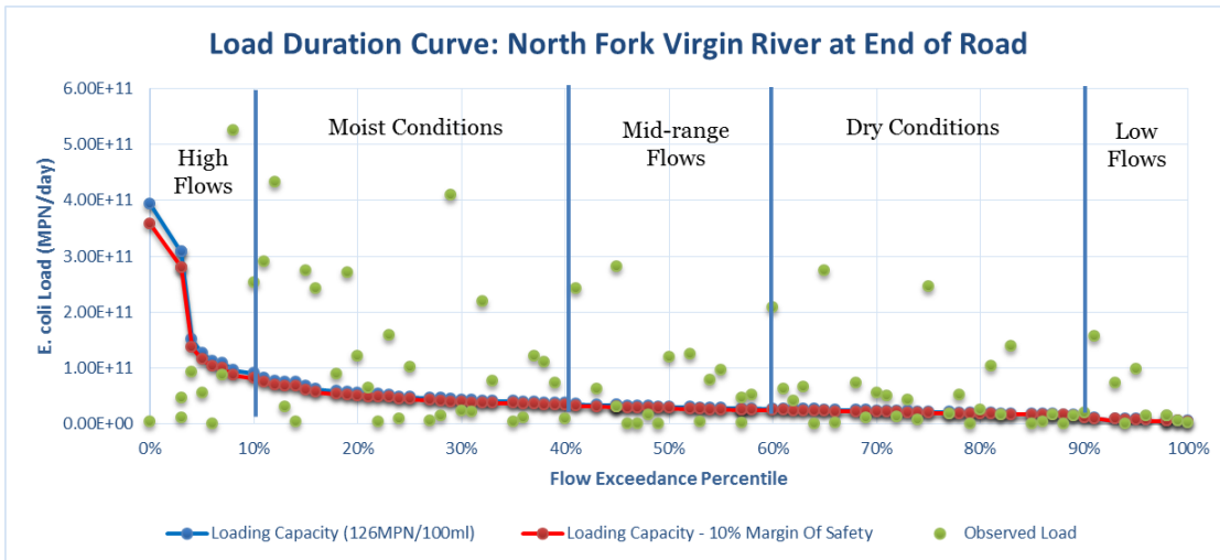
Figure 26: Load duration curve for North Fork Virgin River at End of Road site
