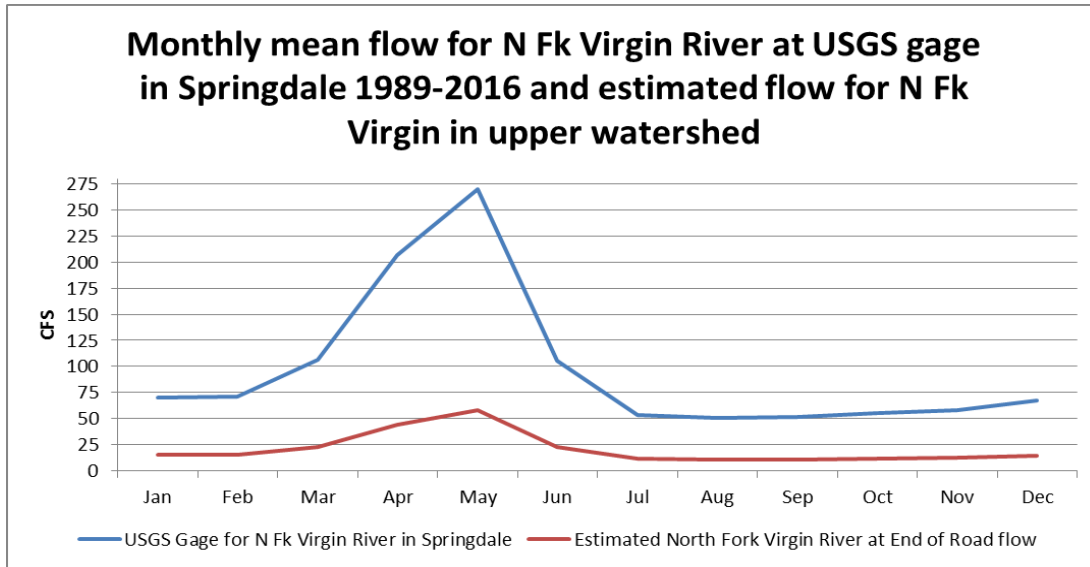
Figure 6: Monthly mean flow (CFS) for North Fork Virgin River in Springdale and estimated flow for North Fork Virgin River at End of Road
