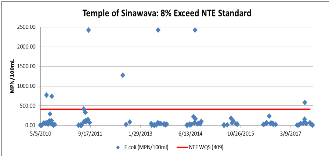
Figure 22: E. coli concentrations in North Fork Virgin River at Temple of Sinawava site above maximum criterion
