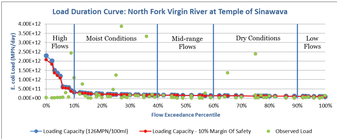
Figure 28: Load duration curve for North Fork Virgin River at Temple of Sinawava
