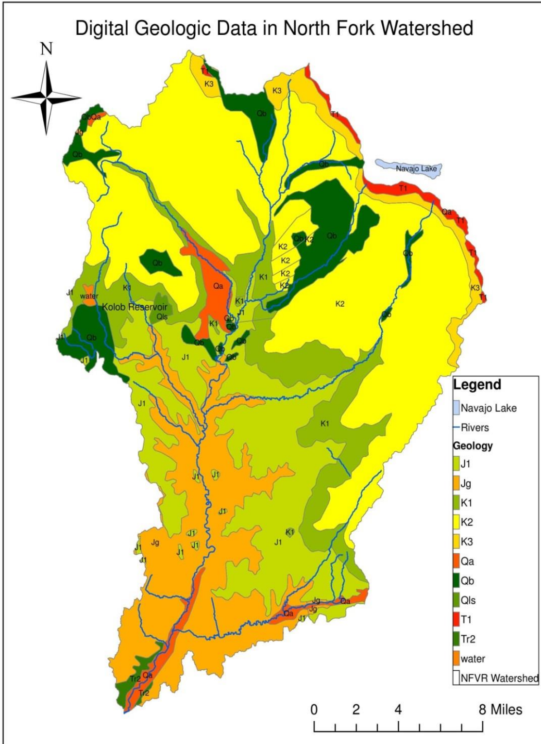
Map 3: Geologic Data in the North Fork Virgin River Watershed (refer to Table 4 below for a description of geologic formation unit symbols)
