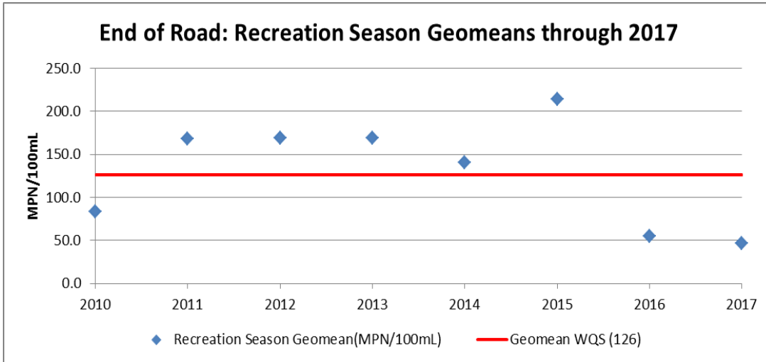
Figure 21: Geometric means of E. coli concentrations during recreation season (May-October) from 2010-2017 at North Fork Virgin River at End of Road site
