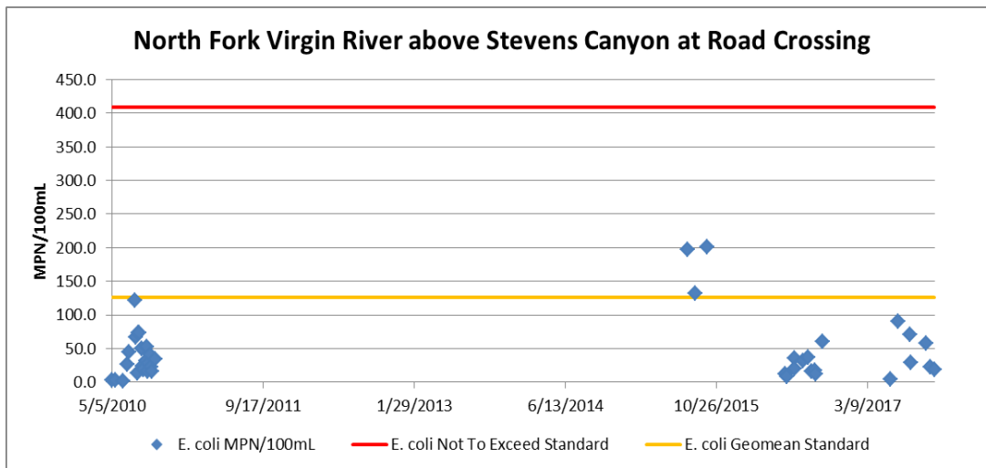
Figure 9: E. coli concentrations measured at North Fork Virgin River above Stevens Canyon at Road Crossing from 2010-2017.
