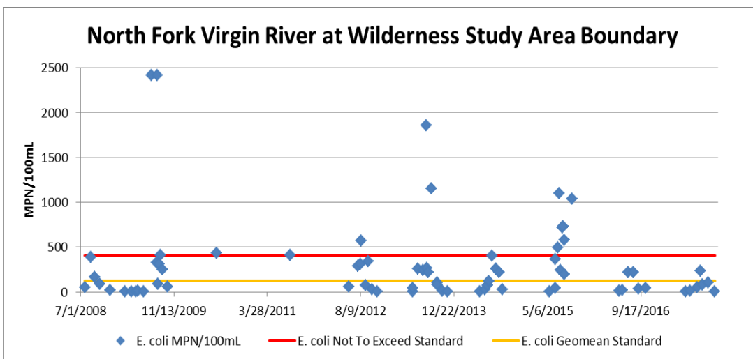
Figure 17: E. coli concentrations measured at North Fork Virgin River at Wilderness Study Area Boundary from 2008-2017.
