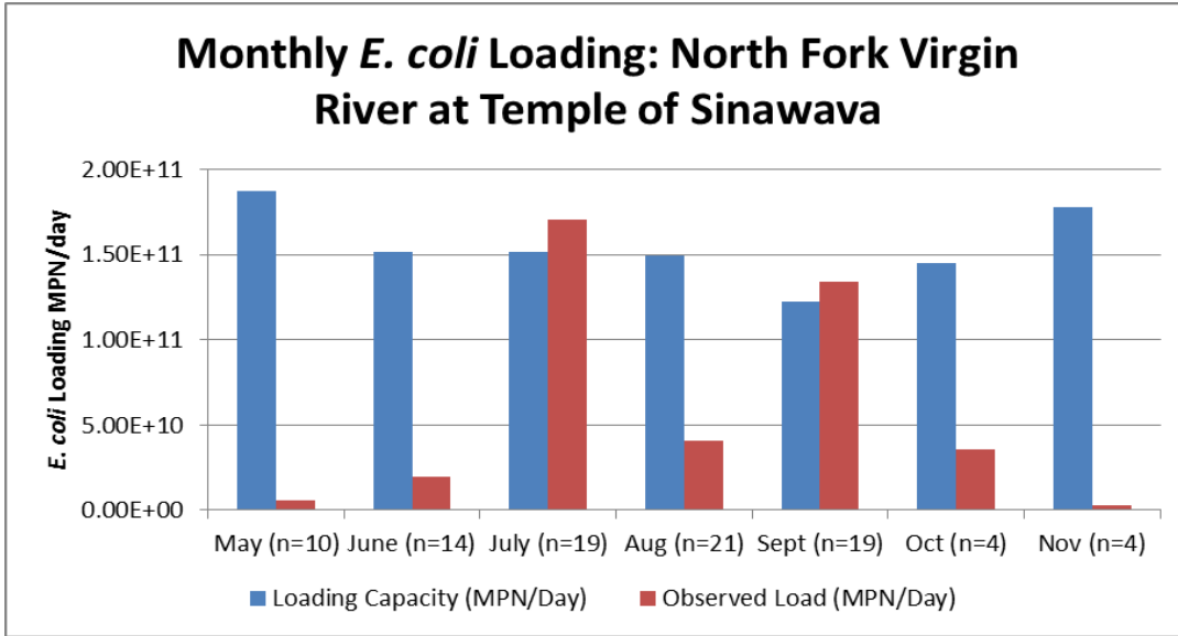
Figure 30: Monthly loading capacity versus observed loading at Temple of Sinawava monitoring site
