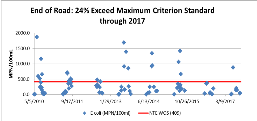
Figure 19: E. coli concentrations above maximum criterion at North Fork Virgin River at End of Road site
