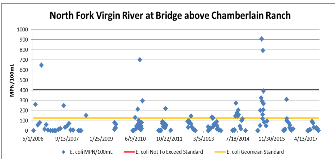
Figure 11: E. coli concentrations measured at North Fork Virgin River bridge above Chamberlain Ranch from 2006-2017.
