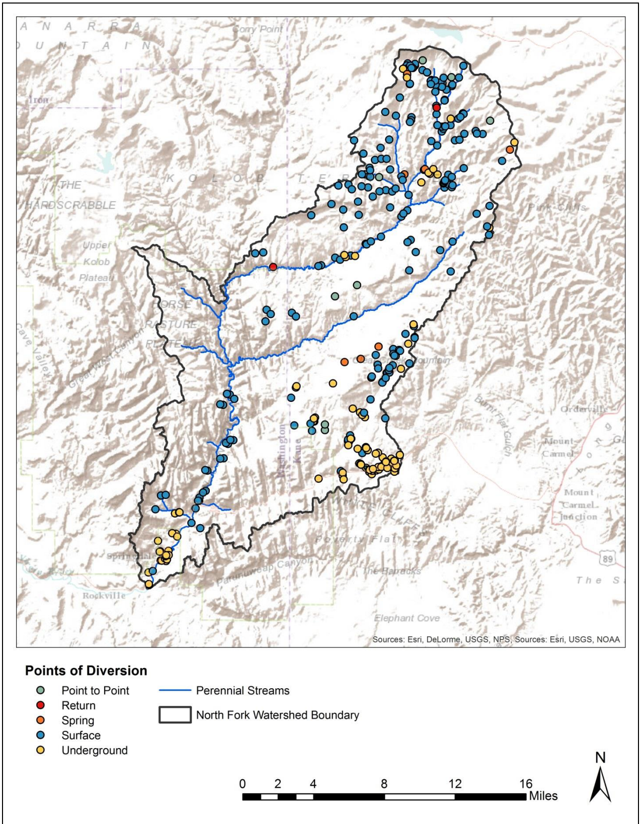
Map 5: Points of diversion in the North Fork Virgin River Watershed.
