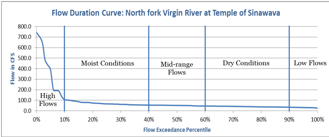
Figure 27: Flow duration curve for North Fork Virgin River at Temple of Sinawava site.
