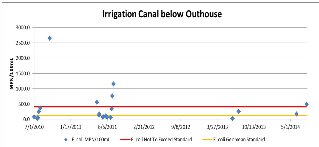
Figure 33: E. coli concentration in the irrigation canal below the outhouse.
