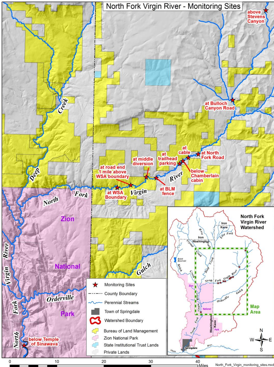
Map 7: North Fork Virgin River monitoring locations
