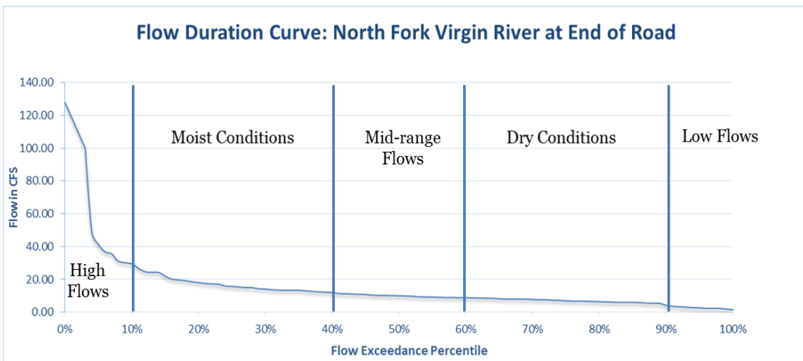
Figure 25: Flow duration curve for the North Fork Virgin River at the End of the Road
