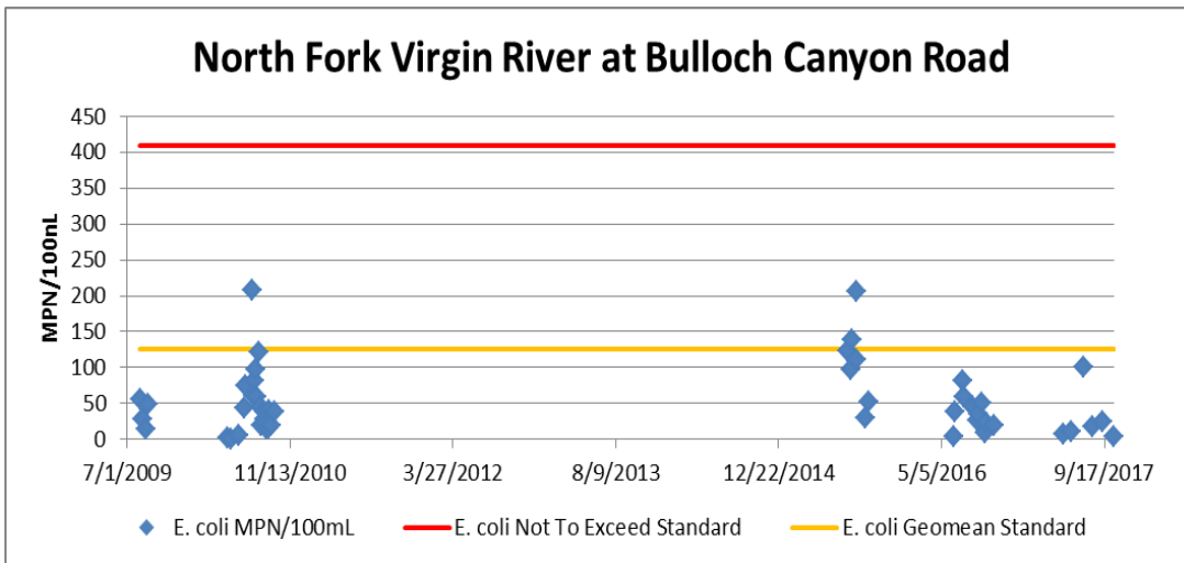
Figure 10: E. coli concentrations measured at North Fork Virgin River at Bulloch Canyon Road from 2009-2017.
