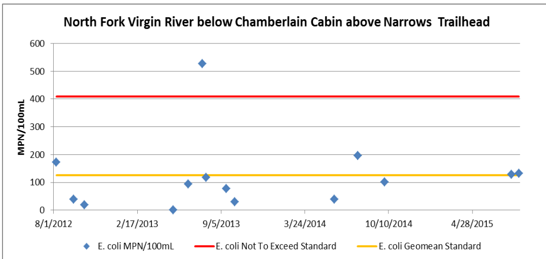
Figure 13: E. coli concentrations measured at North Fork Virgin River below Chamberlain Cabin above Narrows Trailhead from 2012-2015.
